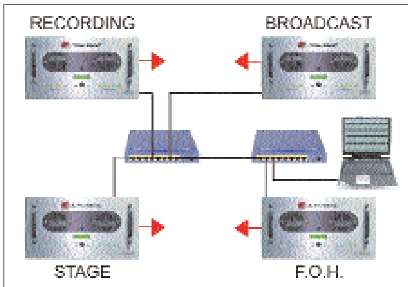
Figure 6: Four ESFs configured for additional broadcast and recording feeds with hardwired splits or analog outputs (red arrows).
