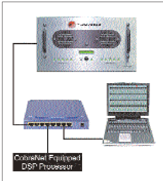
Figure 7: Single ESF used as CobraNet multi-channel I/O access point.
