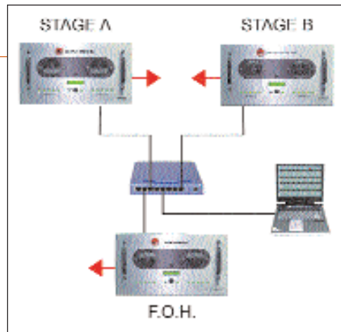
Figure 8: Festival setup with two stage ESFs alternating feeds to a single FOH unit. Presets may be stored to switch instantly between the two stage boxes at changeover. Stage uses analog splits for monitors, FOH has analog output to console (red arrows).
