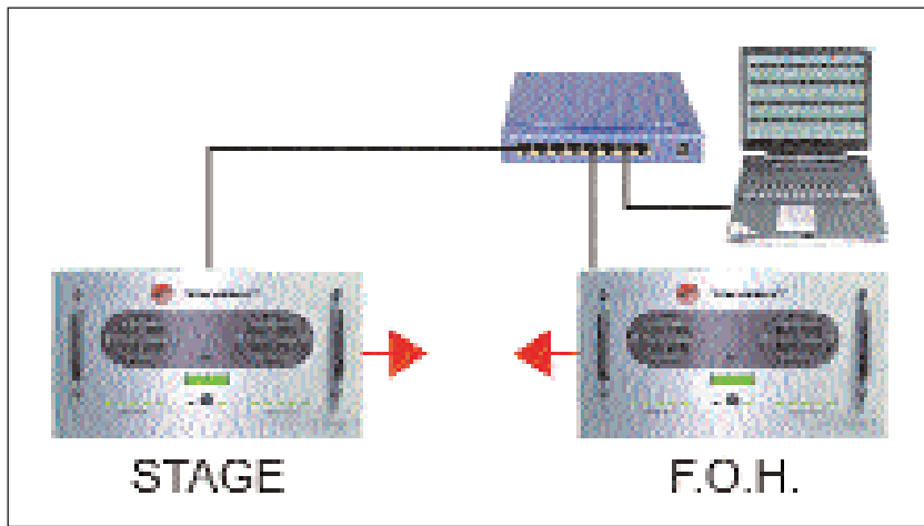
Figure 5: A basic two ESF system with hardwired analog split at stage (monitors) and analog out at FOH (to console), represented by the red arrows.
