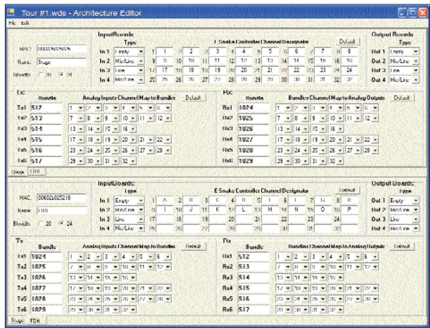
Figure 4: System architecture application.
